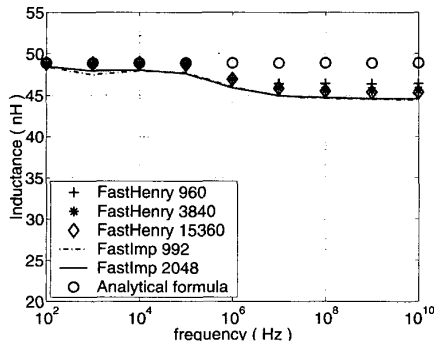
Figure 4: Inductance of a ring
