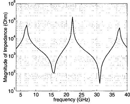
Figure 3: Impedance of a shorted transmission line
