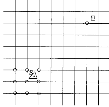
Figure 2: 2-D pictorial representation of the projection step
