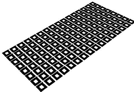
Figure 7: 16x8 3-turn rectangular spiral array
